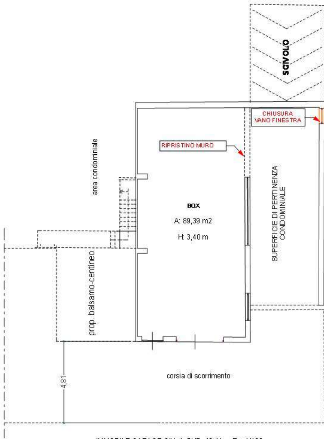
IMMOBILE GARAGE CIV. 4 SUB. 40-41 R= 1/100
